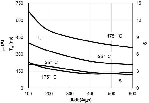
Figure 24: Diode Reverse Recovery Time and Softness Factor vs. di/dt ( V_{GE}=15V , V_{CE}=400V , I_F=50A )
