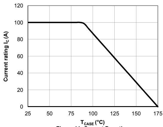
Figure 11: Current De-rating
